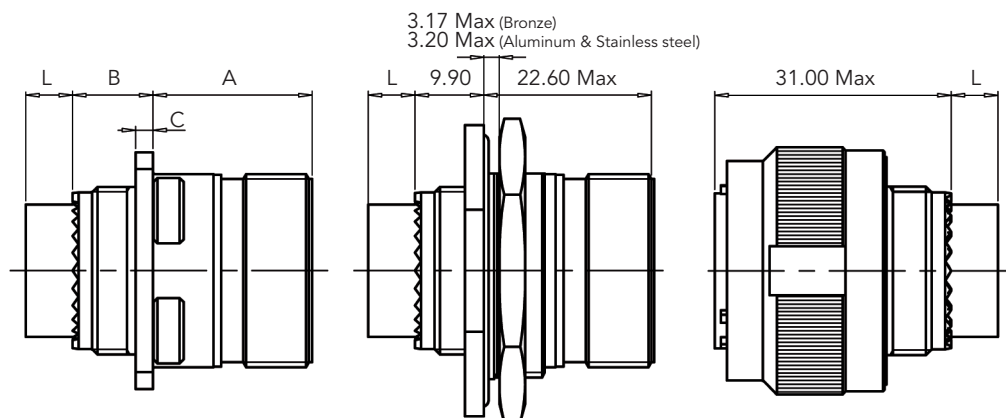
Type 0 Square Flange Receptacle
