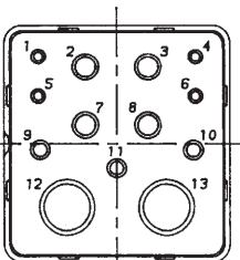
2-11C2 4 size 20 3 size 16 4 size 12 2 coaxial size 5
