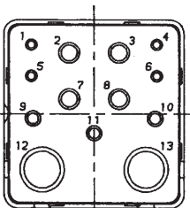
2-11T2 4 size 20 3 size 16 4 size 12 2 triaxial size 8
