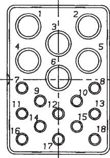
1-C1 2T6 12 coaxial size 12 6 triaxial size 8
