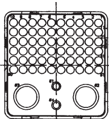
2-62T2 60 size 22 2 size 16 2 triaxial 8
