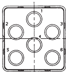
2-T6 6 triaxial size 8 metal insert
