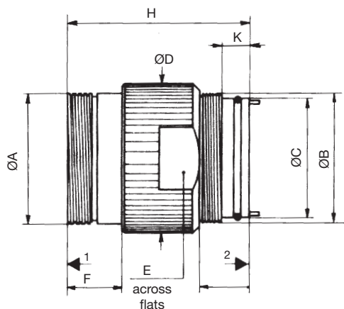
shell size 7
