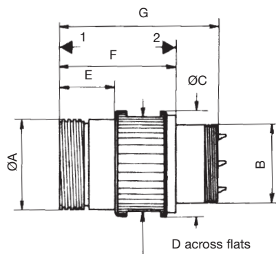
shell sizes 1-4
