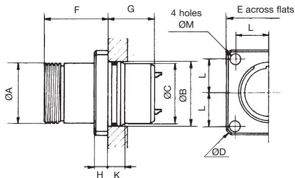
shell size 7
