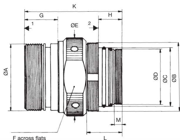
shell size 5-6
