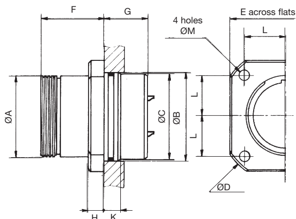
shell size 5-6
