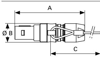
FN - plug straight with lanyard
