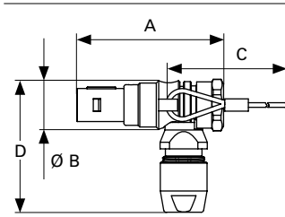
FM - plug right angle plug with lanyard
